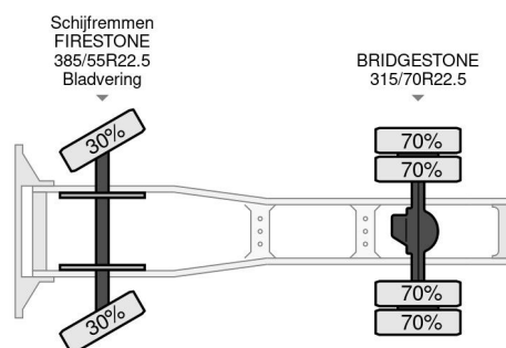
DAF XF 480 FT SUPER SPACE CAB
