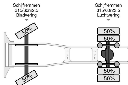
DAF XF 480 FT NGD LOW DECK, different location : T... 4x2
