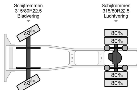
DAF XF 480 FT SPACE CAB , DIFFERENT LOCATION : ... 4x2
