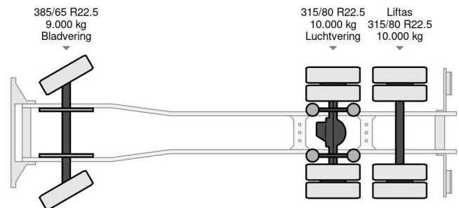
DAF CF 480 FAS Containerhook LC TAM T22
