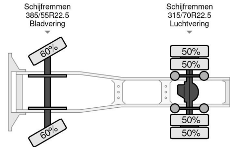
DAF XF 480 FT SUPER SPACE CAB ZF INTARDER 4x2 Referentienummer: 0G379914
