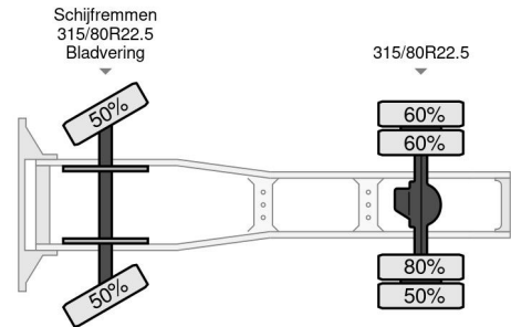
DAF CF 450 FT SPACE CAB
