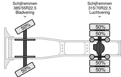
DAF XF 480 FT SUPER SPACE CAB ZF INTARDER 4x2 Referentienummer: 0G383598
