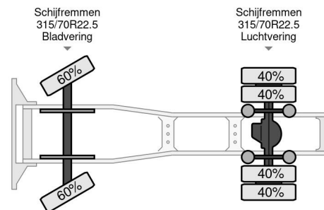
DAF XF 480 FT SPACE CAB
