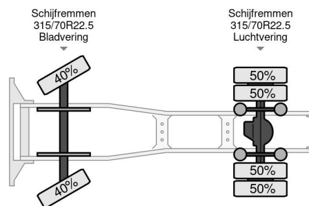
DAF XF 440 FT SUPER SPACE CAB
