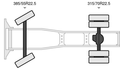
DAF XF 480 FT SUPER SPACE CAB ADR 4x2 Referentienummer: 0G340173
