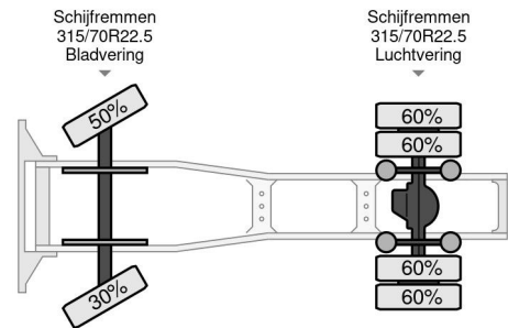
DAF XF 450 FT SPACE CAB ADR
