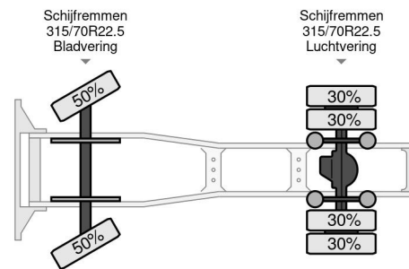
DAF XF 450 FT SPACE CAB ADR
