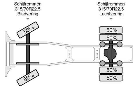
DAF XF 440 FT SPACE CAB ADR
