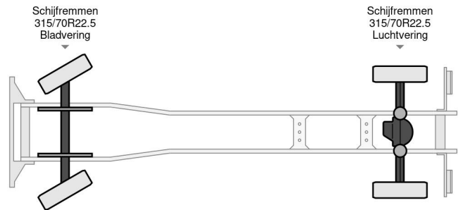
DAF CF 290 FA
