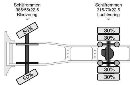
DAF XF 480 FT SUPER SPACE CAB ZF INTARDER 4x2 Referentienummer: 0G273213
