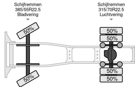
DAF XF 460 FT SUPER SPACE CAB
