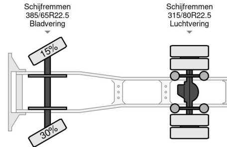
DAF XF 480 FT SUPER SPACE CAB ZF INTARDER 4x2 Referentienummer: 0G323343
