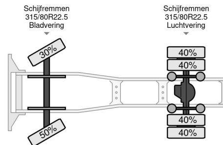
DAF XF 480 FT SUPER SPACE CAB ZF INTARDER 4x2 Referentienummer: 0G180043
