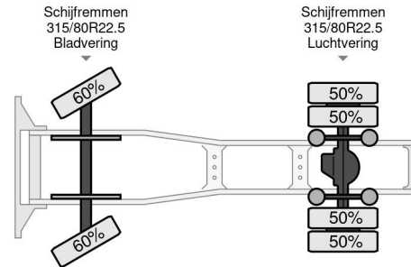
DAF XF 460 FT SPACE CAB ZF INTARDER
