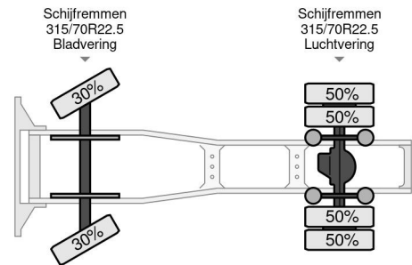
DAF XF 480 FT SPACE CAB ADR ZF INTARDER 4x2 Referentienummer: 0G316094
