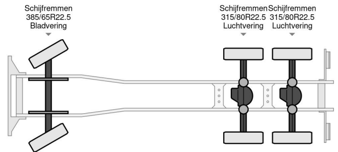
DAF CF 530 FTT WITH CRANE EPSILON PALFINGER... 6x4
