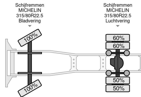
DAF XF 530 FT SPACE CAB
