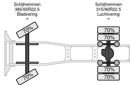
DAF XF 480 FT SUPER SPACE CAB ADR 4x2 Referentienummer: 2-DGN-687
