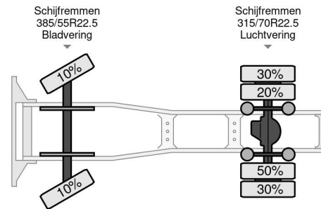
DAF XF 530 FT SPACE CAB
