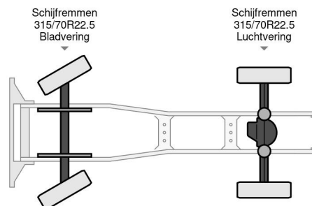
DAF XF 480 FT NGD , different location : TRUCK TRAD... 4x2
