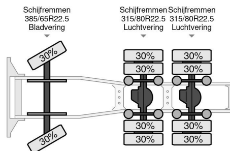
DAF XF 530 FTT SPACE CAB ZF INTARDER
