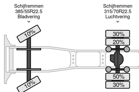
DAF XF 530 FT SPACE CAB
