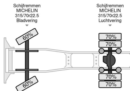
DAF XF 480 FT SUPER SPACE CAB ZF INTARDER , D... 4x2
