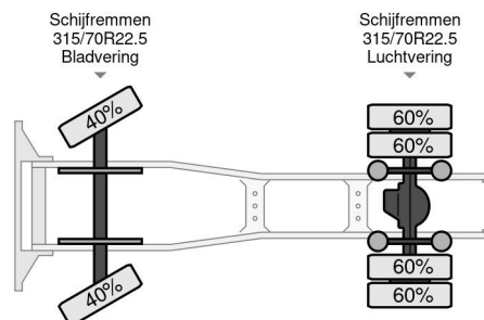
DAF XF 480 FT SPACE CAB , different location : TRUC... 4x2 Referentienummer: 0G279727
