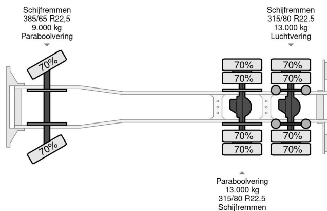
DAF CF 480 FAT 6x4 with AJK hooksystem for containers - ret...
