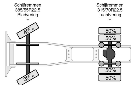
DAF XF 480 FT SUPER SPACE CAB ZF INTARDER
