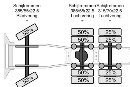
DAF XF 480 FTG SUPER SPACE CAB ZF INTARDER 6x2
