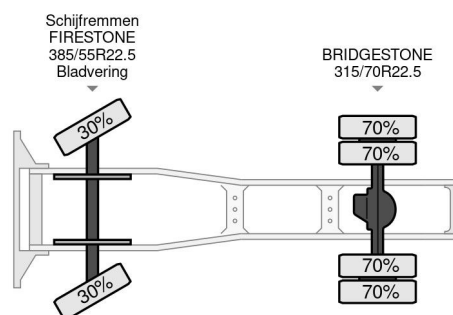
DAF XF 480 FT SUPER SPACE CAB
